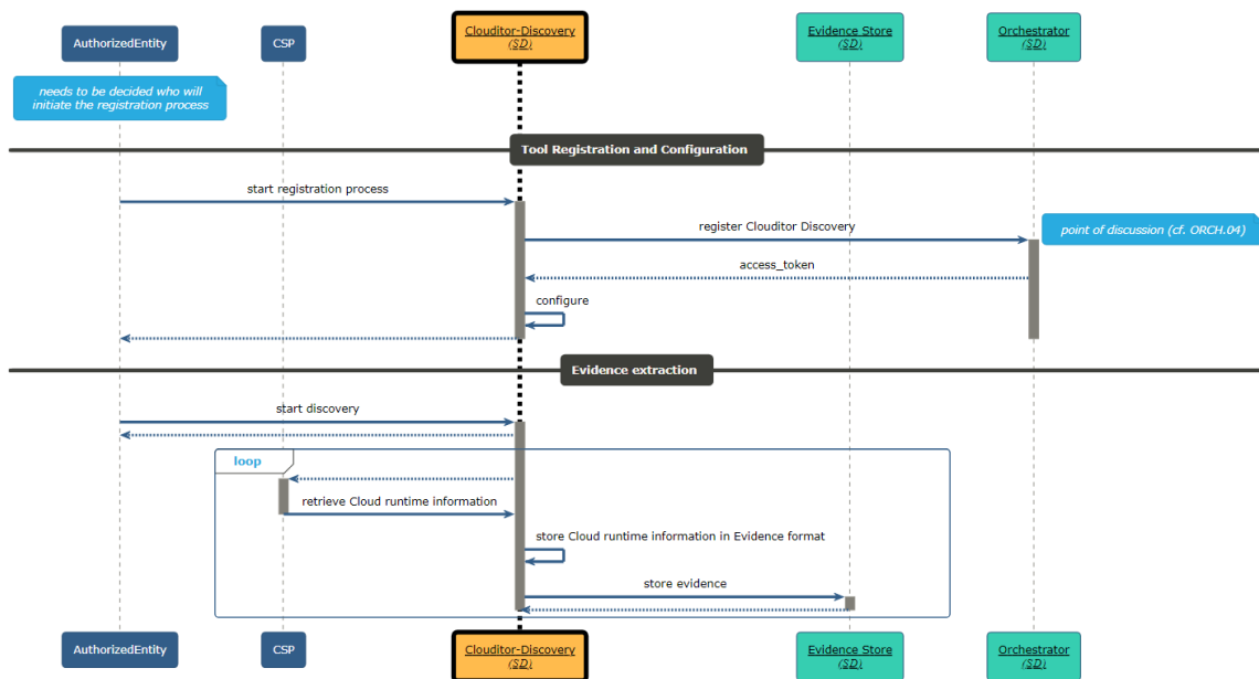
Figure 11. Clouditor-Discovery sequence diagram
