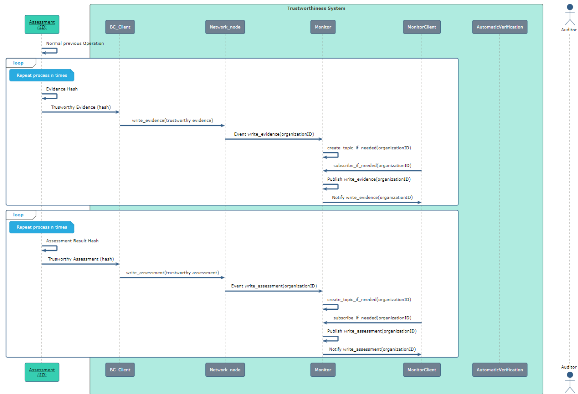
Figure 15. TWS System Recording sequence diagram
