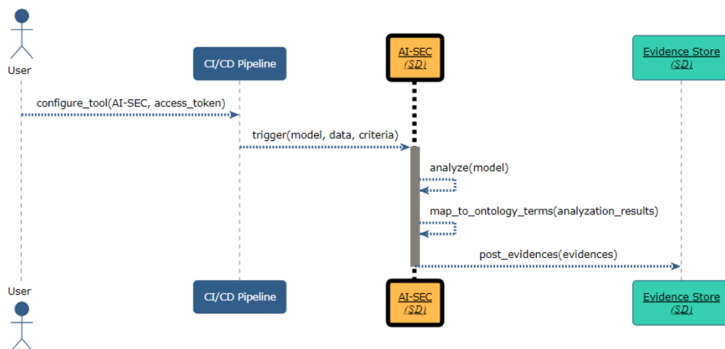
Figure 9. AI-SEC sequence diagram
