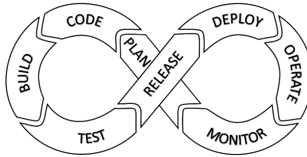
Figure 1. DevOps Cycle
