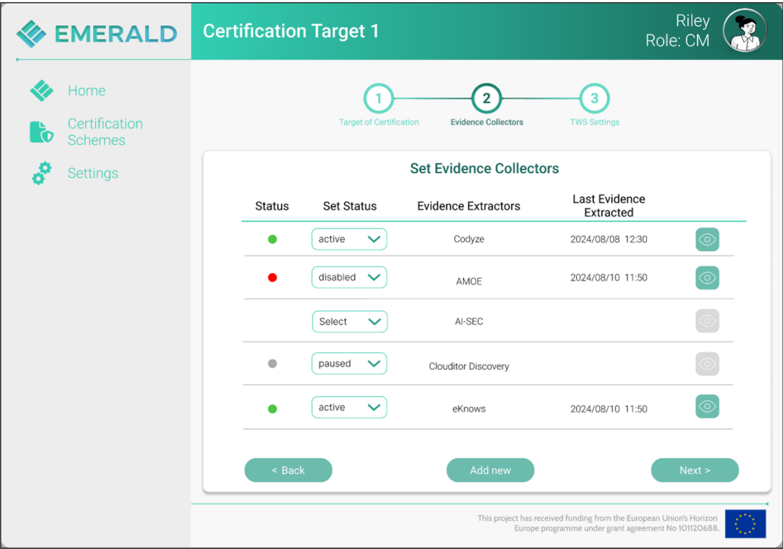
Figure 3. Configuration of evidence collectors in the EMERALD UI (D4.3 [14])
