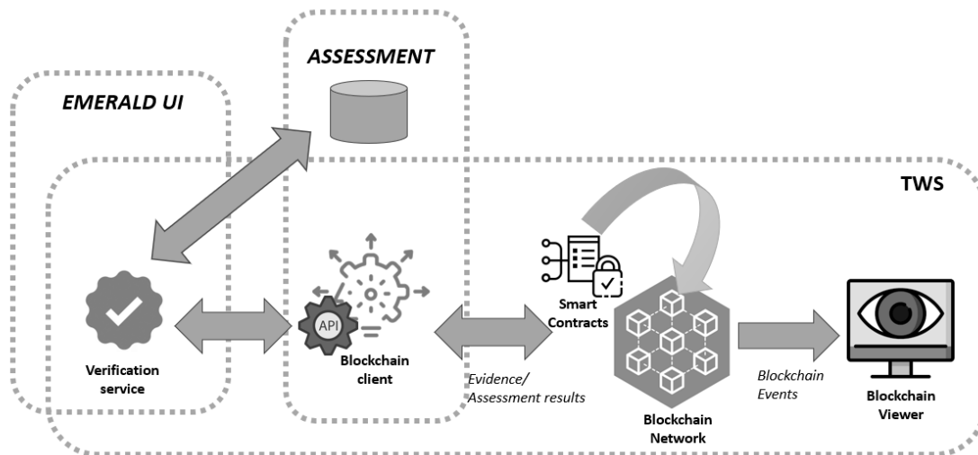
Figure 31. TWS architecture
